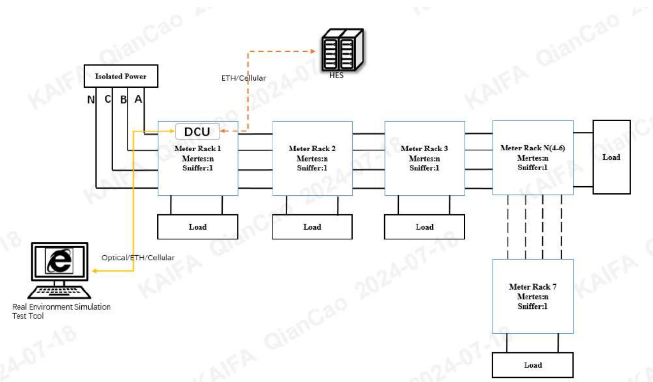
Figure 3-23 Test Setup for PLC Network Performance Test
