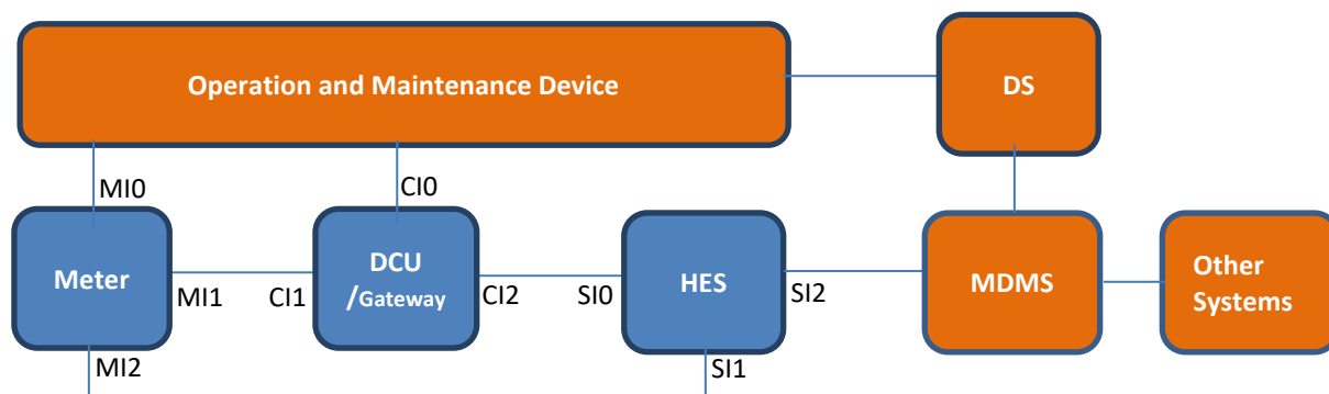
Figure 1: Interface Architecture
