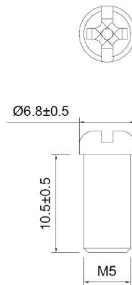
Figure - Dimensions of terminal screw
