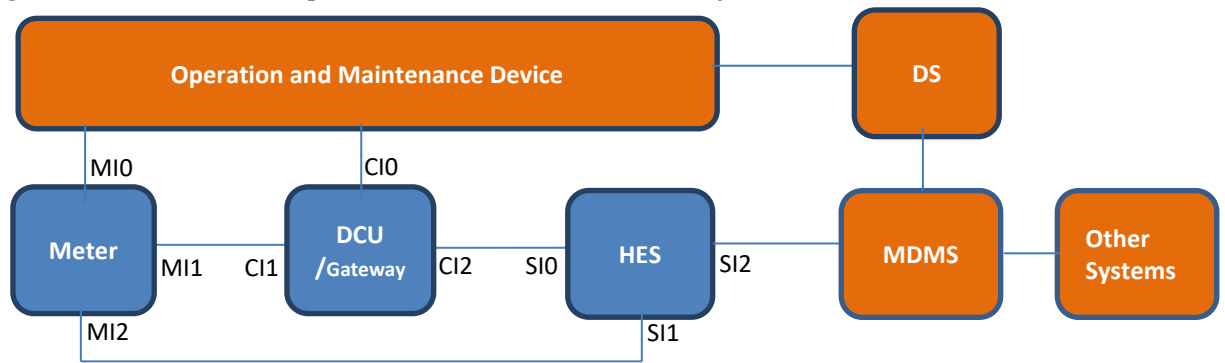
Figure 2: System and Interface Architecture
