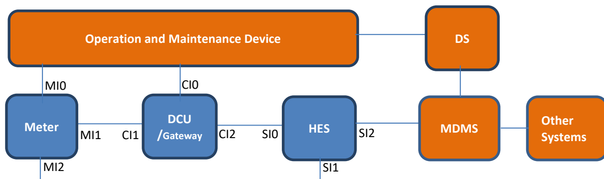
Figure 1: Interface Architecture
