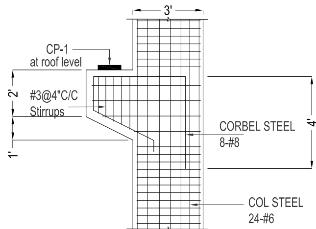
DETAIL "1"
