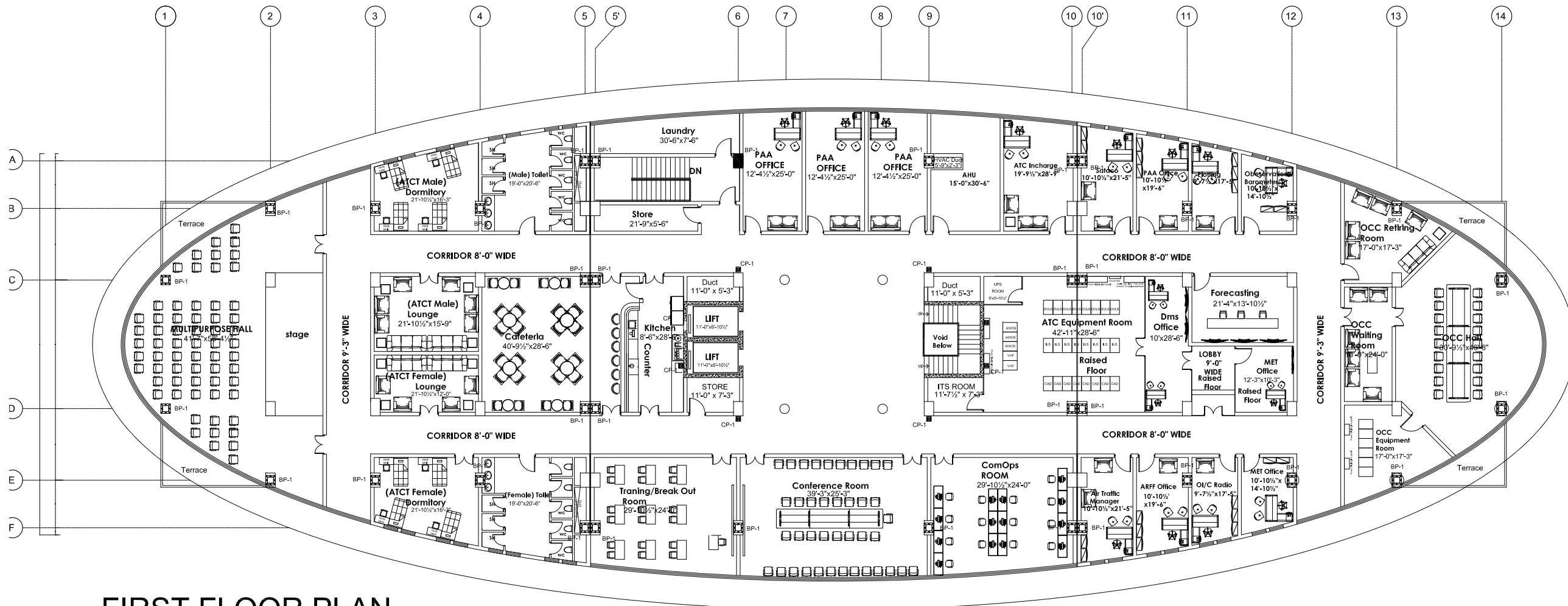
FIRST FLOOR PLAN Covered Area = 27439 Sft
