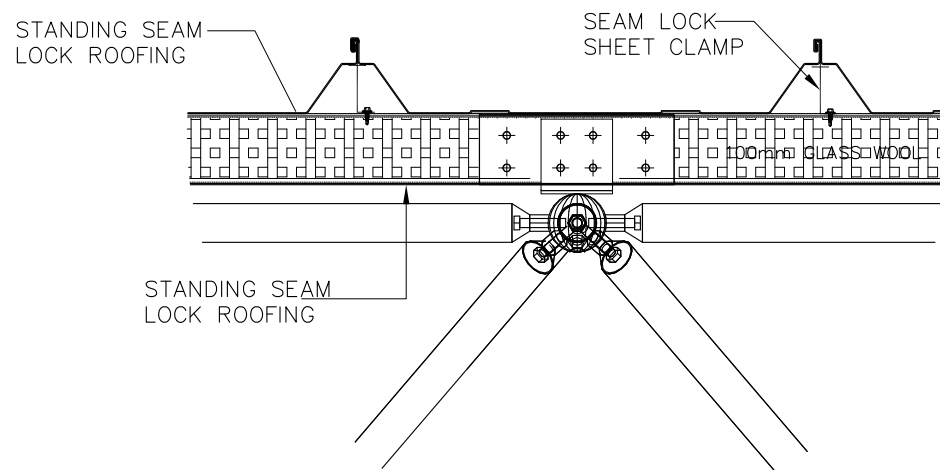
ROOF SHEET DETAIL
