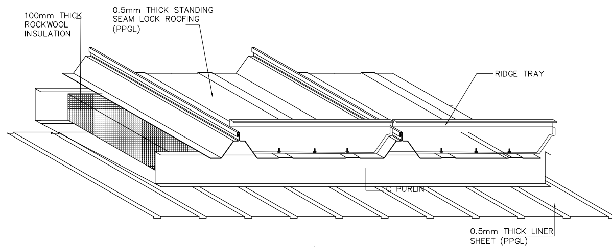
ROOF SHEET AT RIDGE
