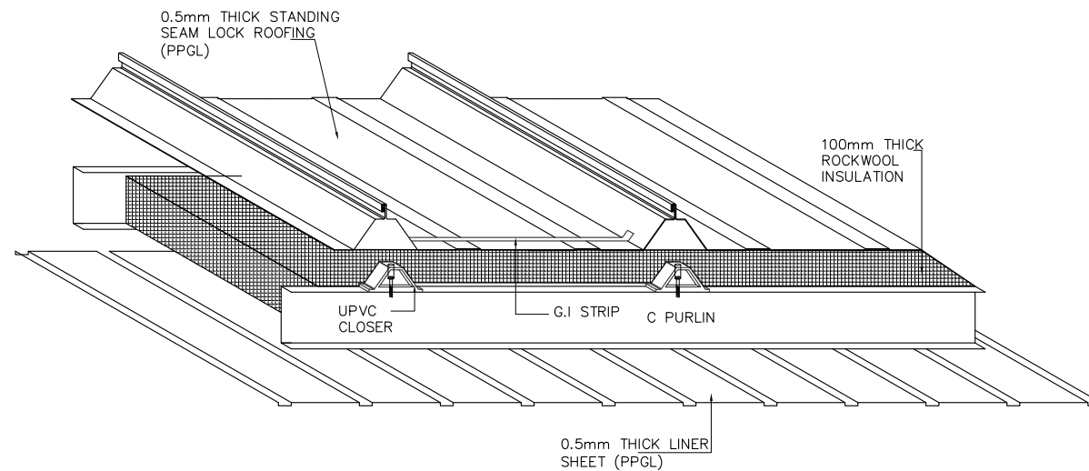
ROOF SHEET AT EAVE
