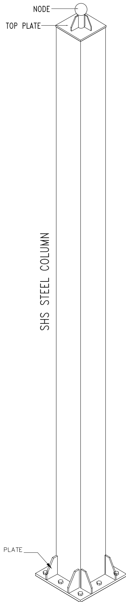
STEEL COLUMN
