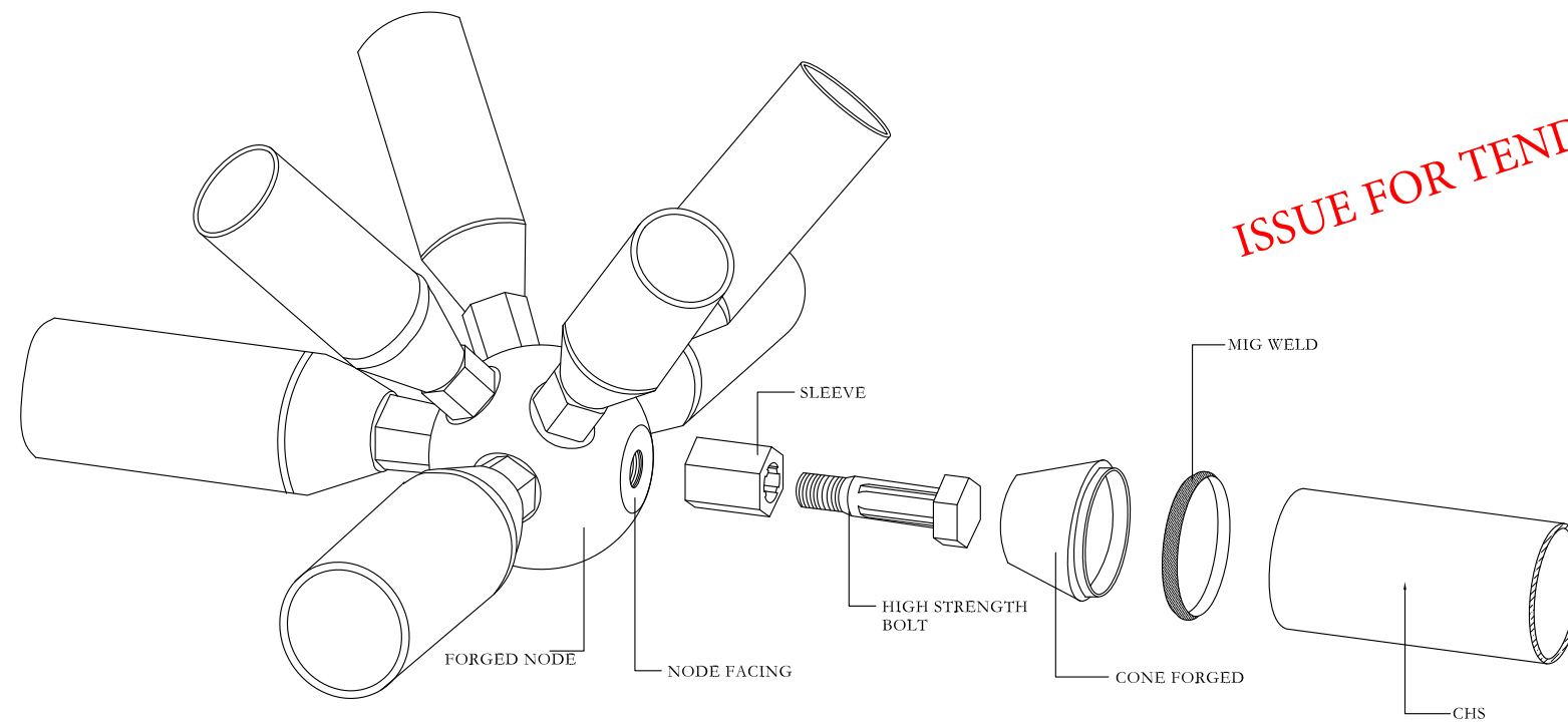
CORD CONNECTION DETAIL
