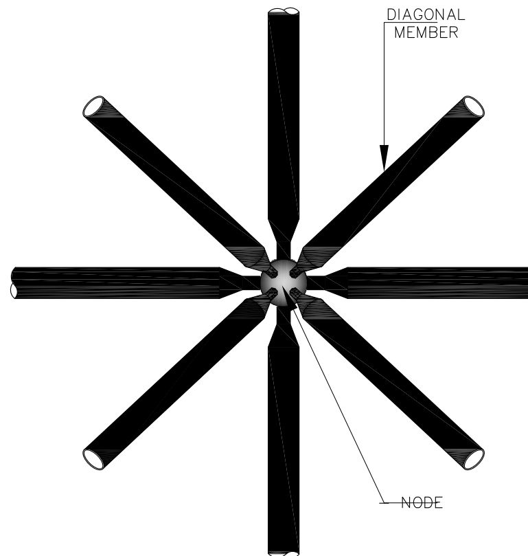
CORD CONNECTION PLAN
