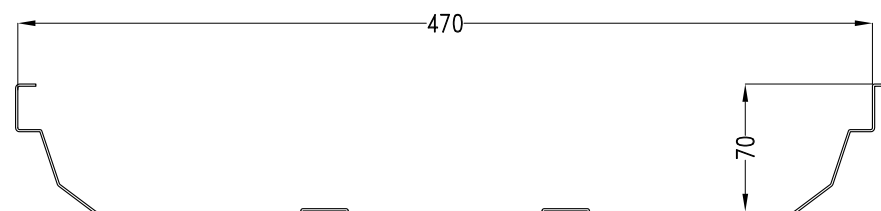
STANDING SEAM LOCK SHEET PROFILE
