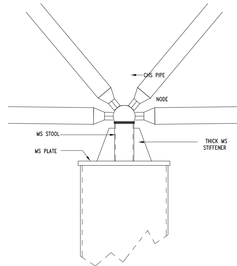
SUPPORTING COLUMN DETAIL
