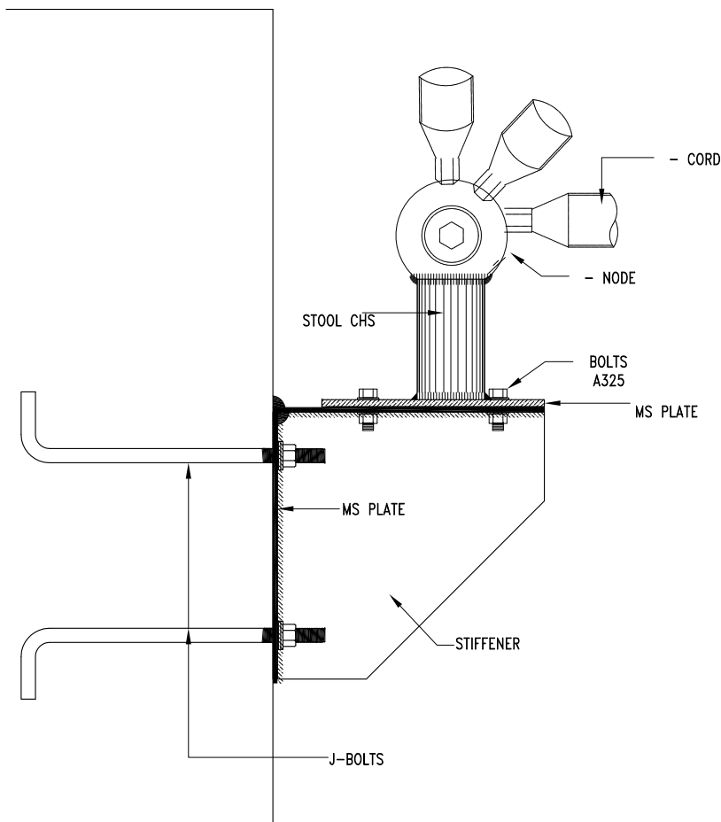
CONNECTION PLATE -1 (CP-1)
