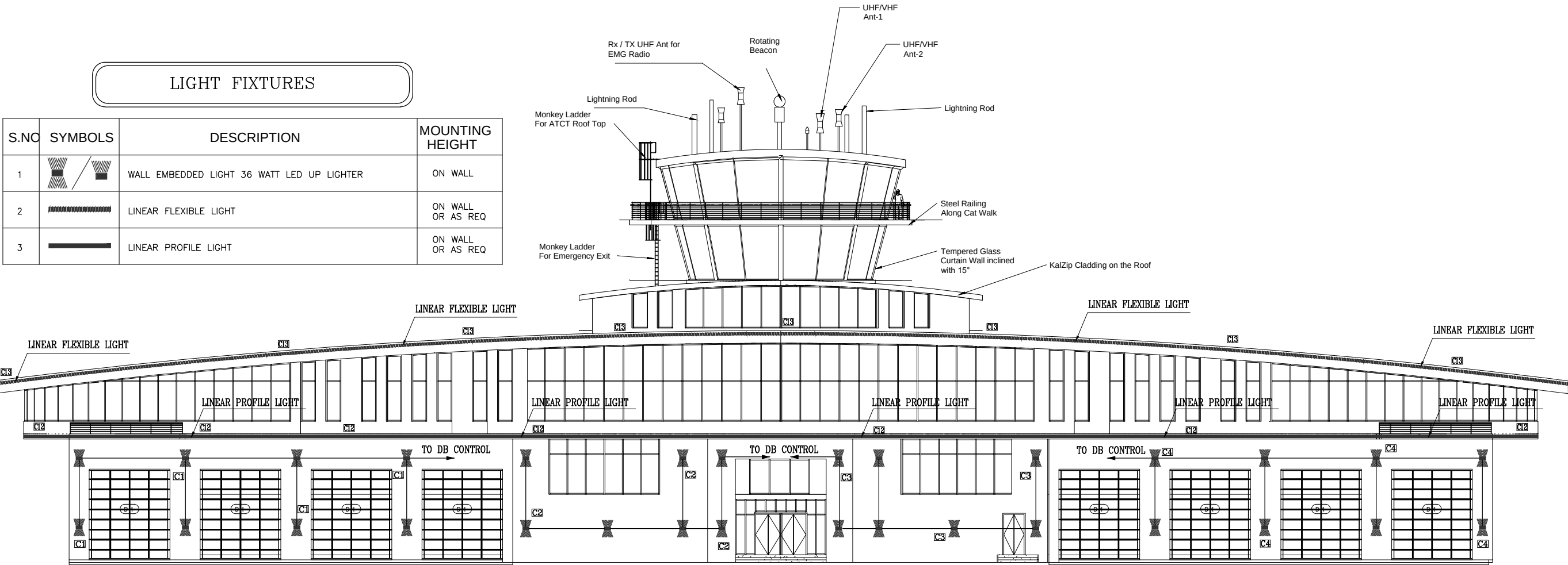
Front Elevation
