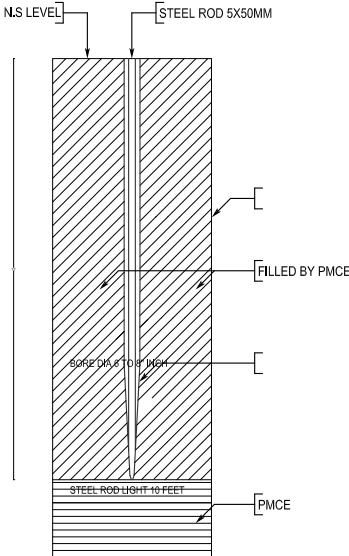
EARTHING DETAIL
