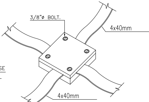
ISOMATRIC VIEW.
