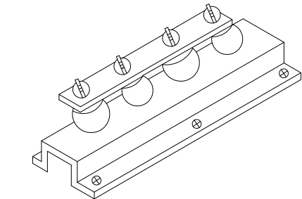
DISCONNECTING LINK
