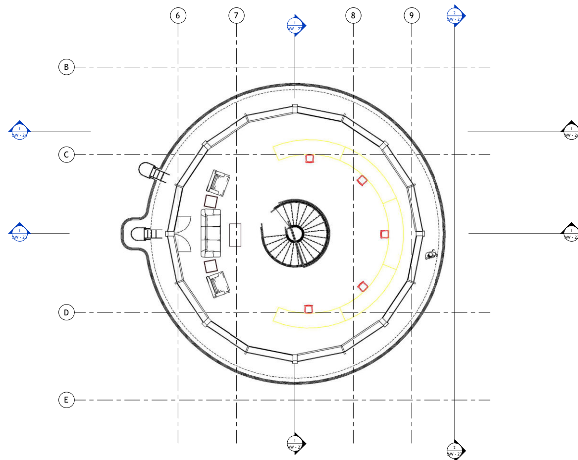
① ATCT CONTROL CABIN PLAN 3/16" = 1'-0"
