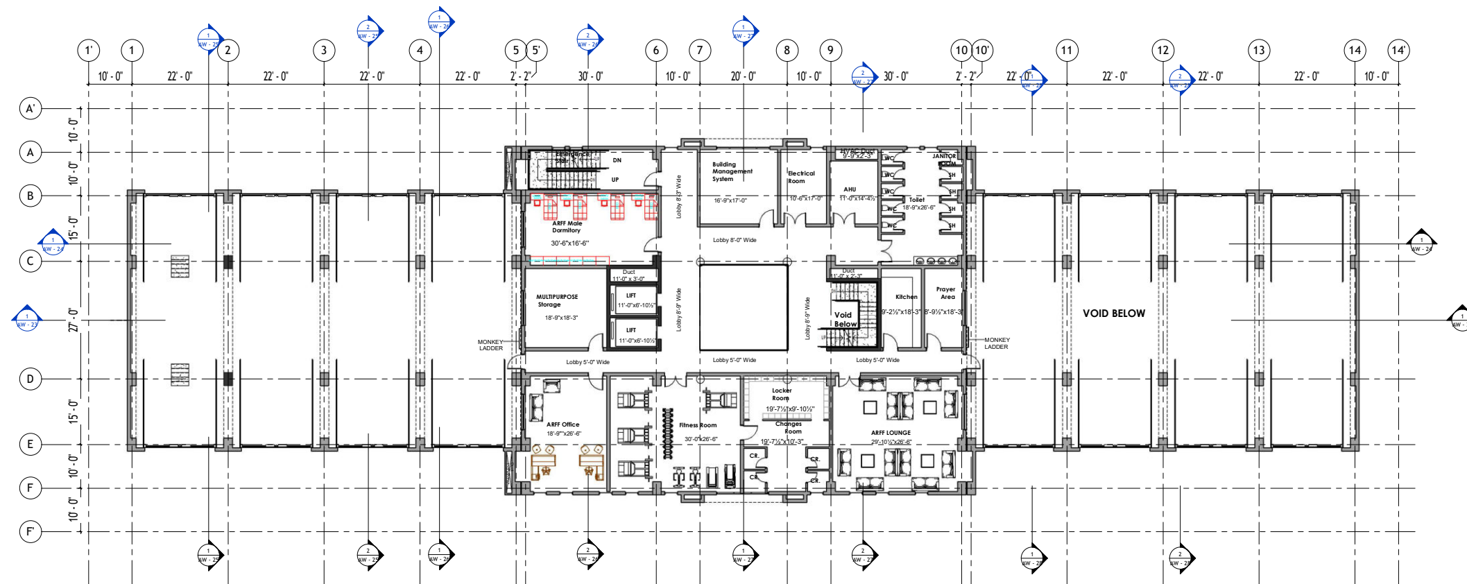
MEZZANINE FLOOR PLAN (ARFF) 1" = 10'-0"
