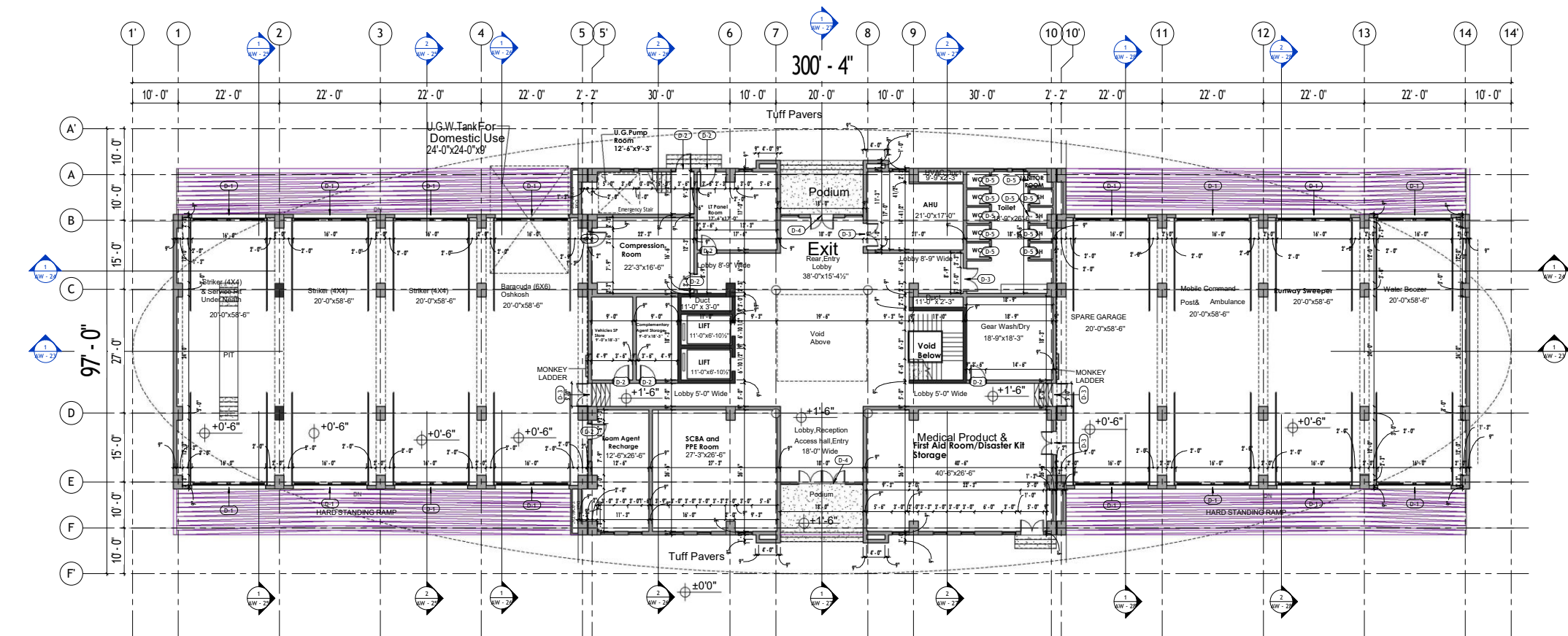
GROUND FLOOR WORKING PLAN 1" = 10'-0"
