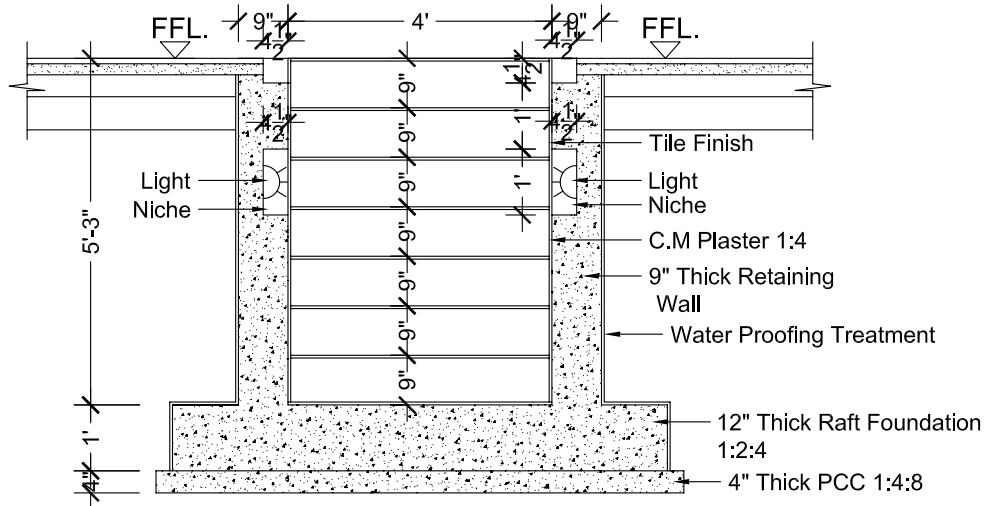
PIT SECTION 5-5
