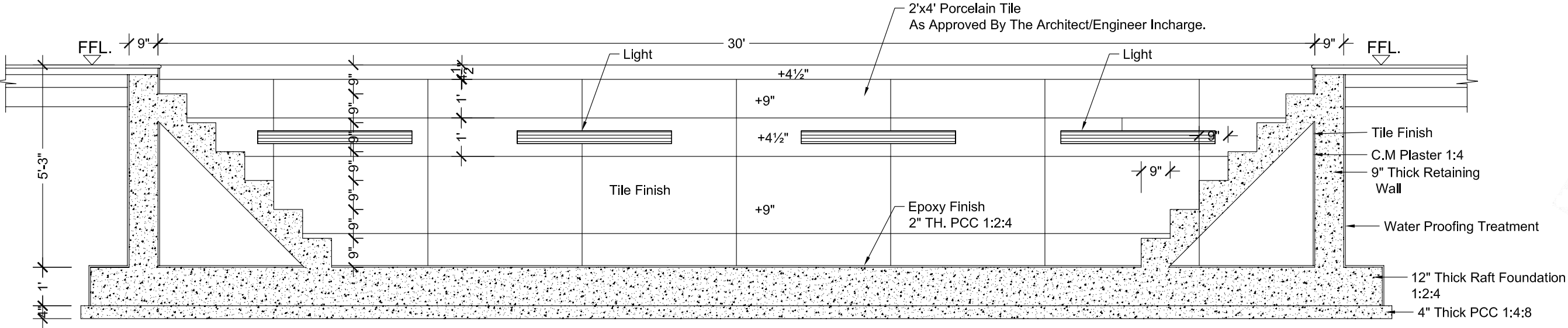
PIT SECTION 4-4
