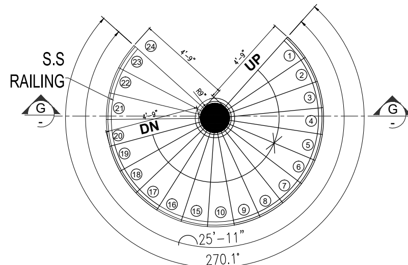
MS STAIR ARFF Control Cabin Level At +56' - 0" NO.OF STEPS = 24 WIDTH = 4'-9" TREAD = 10" RISER= 6 "
