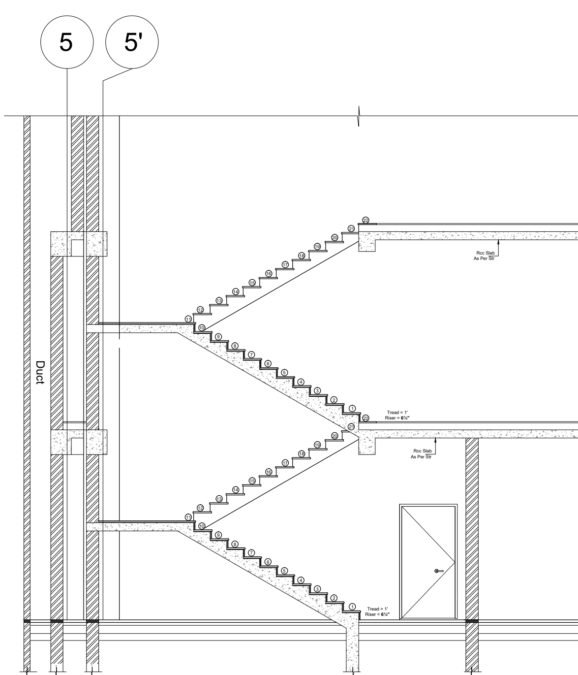
Section at F-F
