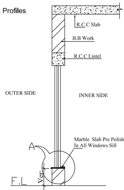
TYPICAL DETAIL OF MARBLE SLAB
