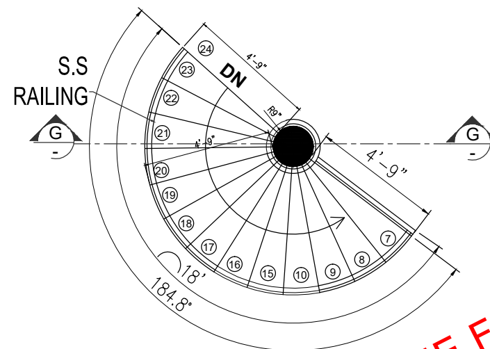
MS STAIR ATCT Control Cabin Level At +68' - 0"
