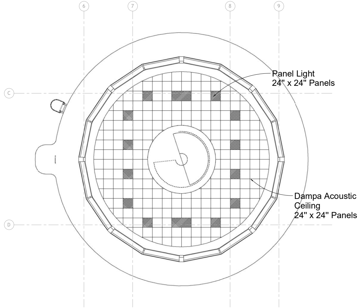
① ARFF CONTROL CABIN PLAN 1/4" = 1'-0"
