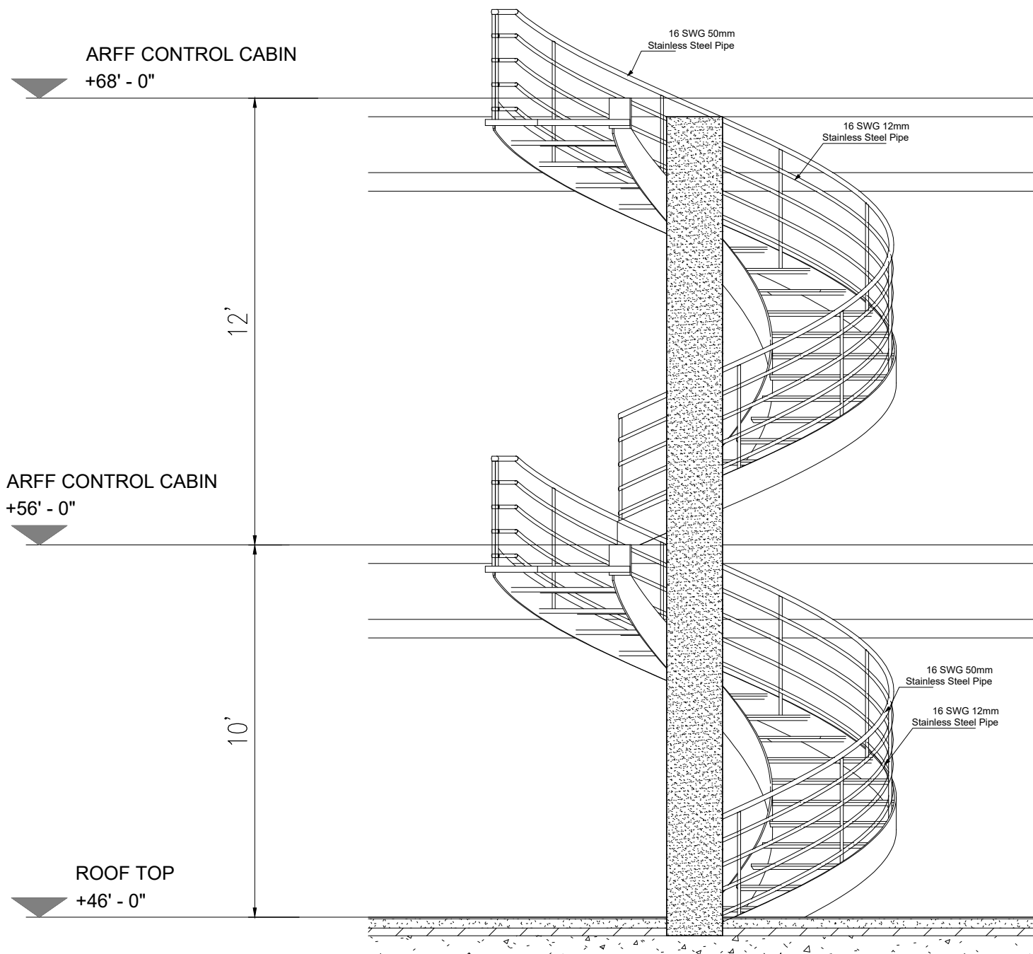
Section at G-G
