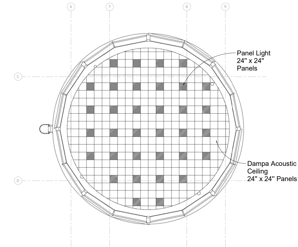
① ATCT CONTROL CABIN PLAN 1/4" = 1'-0"
