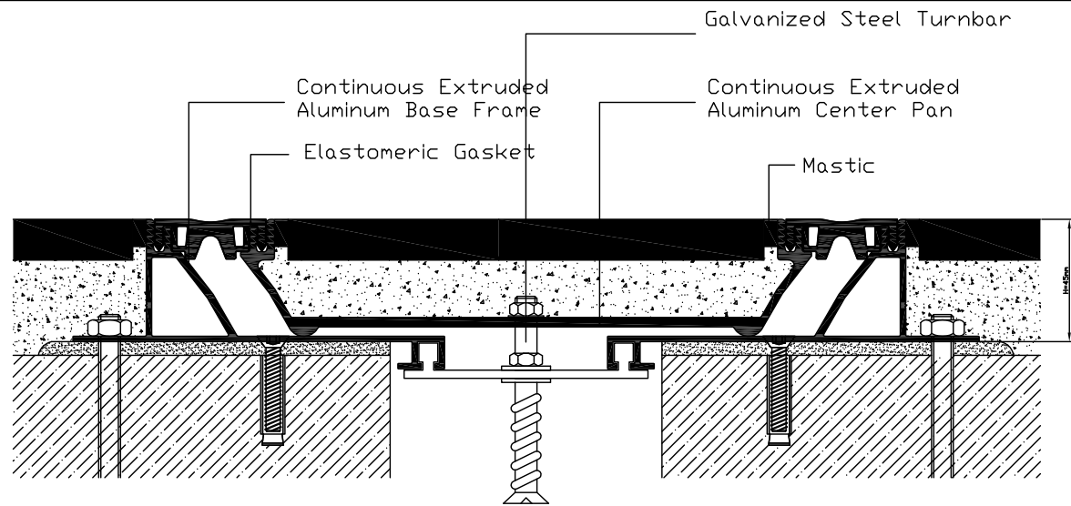
Seismic Floor Joint Profiles
