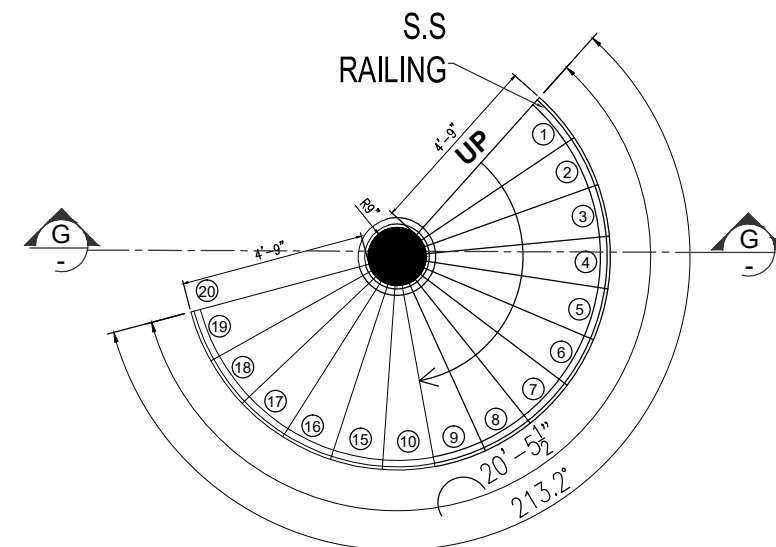
MS STAIR Roof Plan Level At +46' - 0" NO.OF STEPS = 20 WIDTH = 4'-9" TREAD = 10" RISER= 6 "
