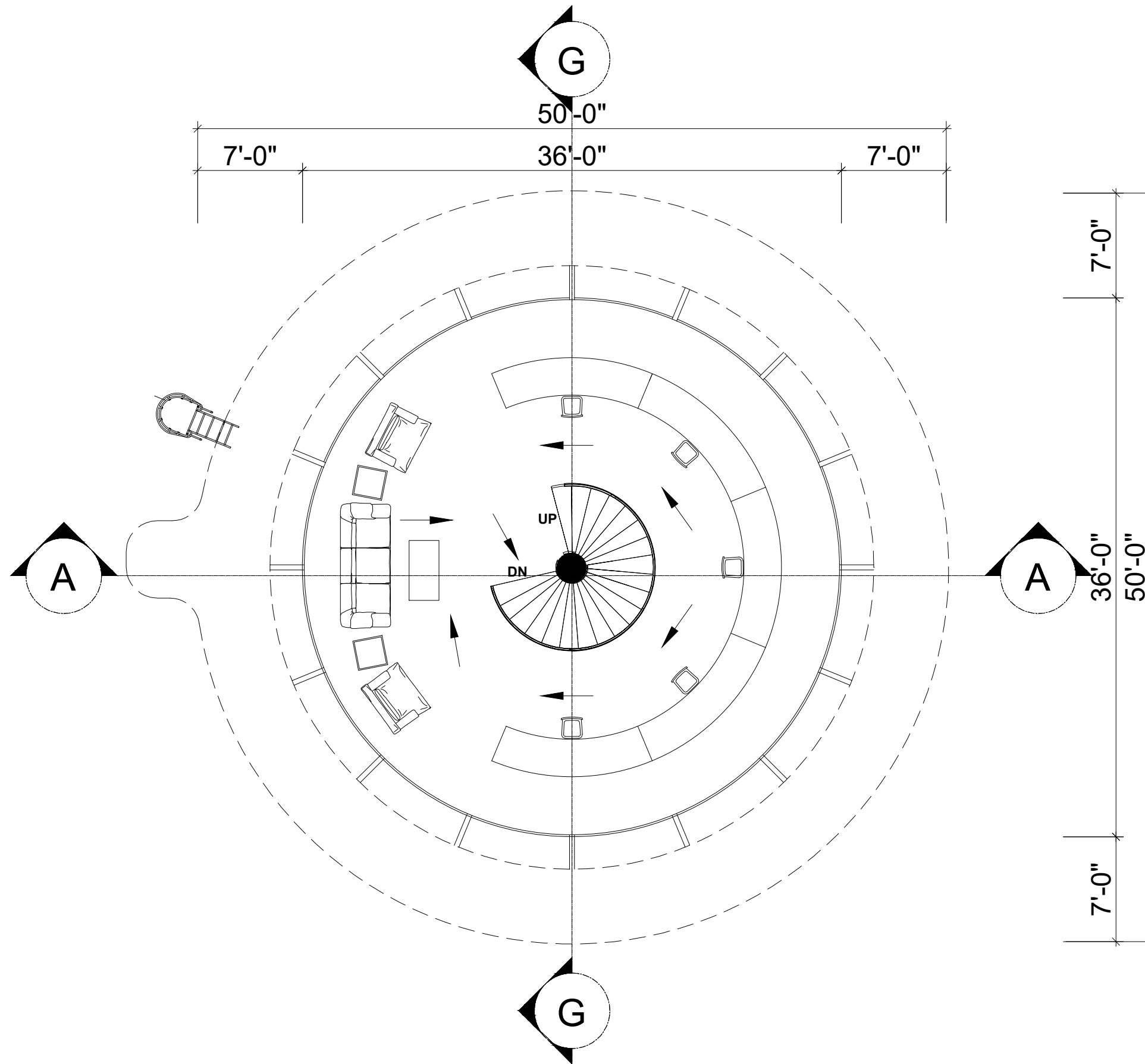
ARFF FLOOR PLAN LEVEL AT 56'-0" COVERED AREA 1277 Sft
