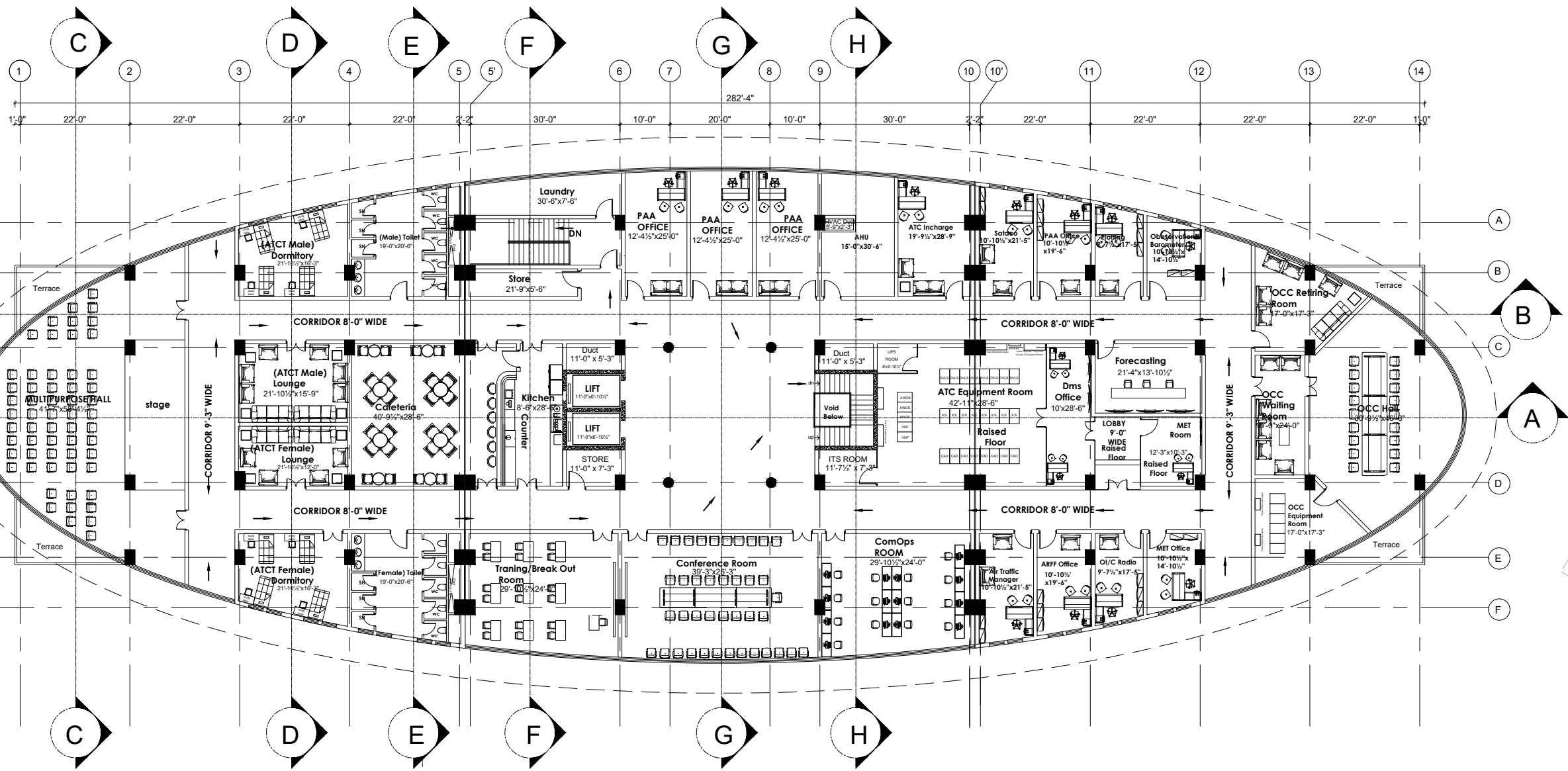
FIRST FLOOR PLAN Covered Area = 27439 Sft
