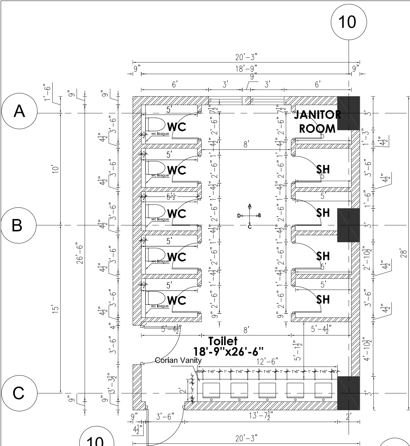
MEZZANINE FLOOR TOILET PLAN
