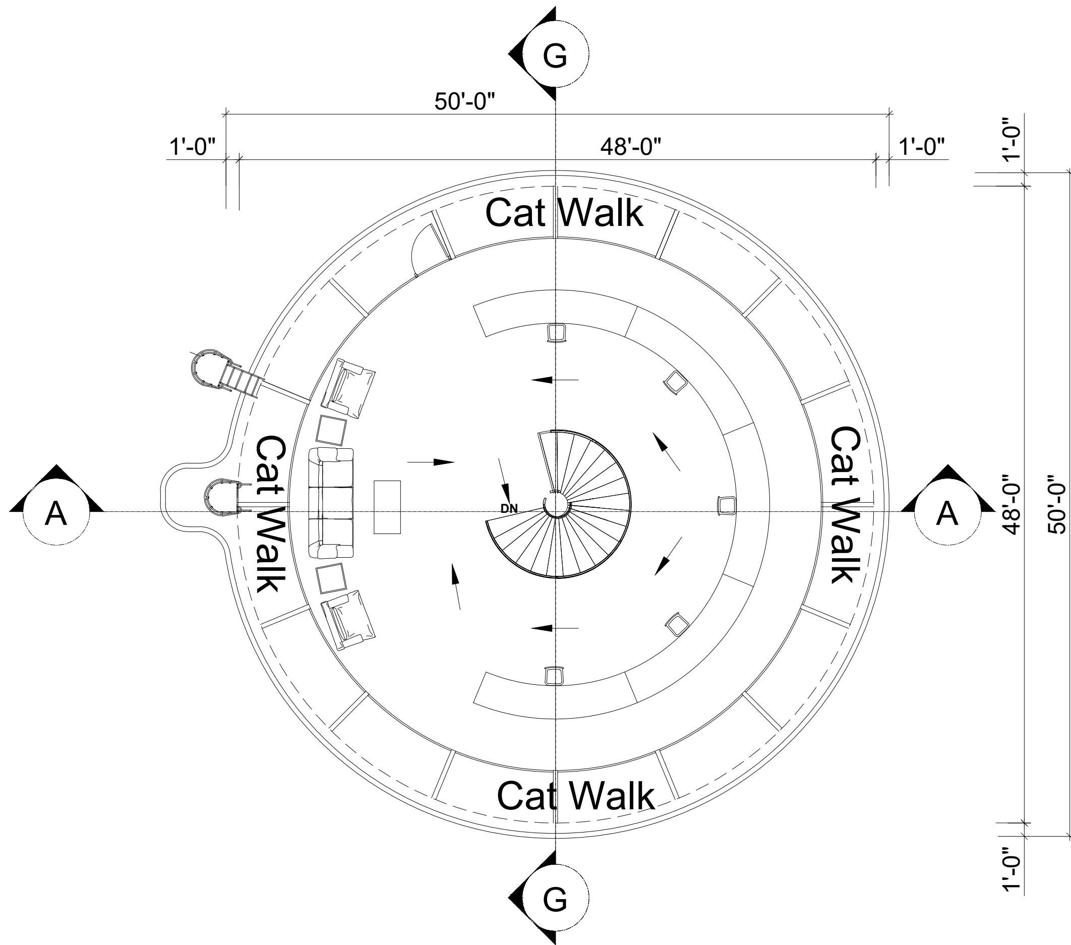
ATCT FLOOR PLAN LEVEL AT 68'-0" COVERED AREA 1809 Sft
