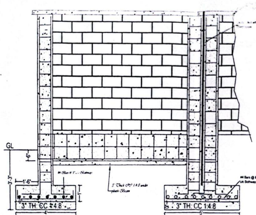
Elevation of Wall
