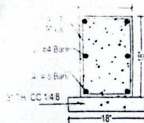
Plinth Beam
