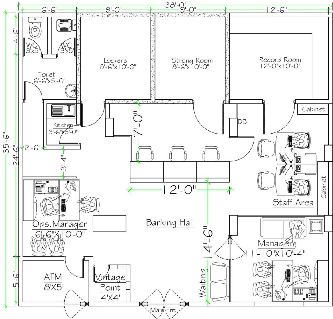
GROUND FLOOR (Proposed) Total Area = 1349 SFT
