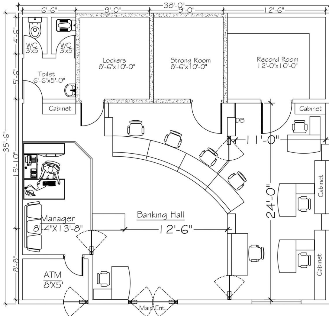
GROUND FLOOR (Existing) Total Area = 1349 SFT
