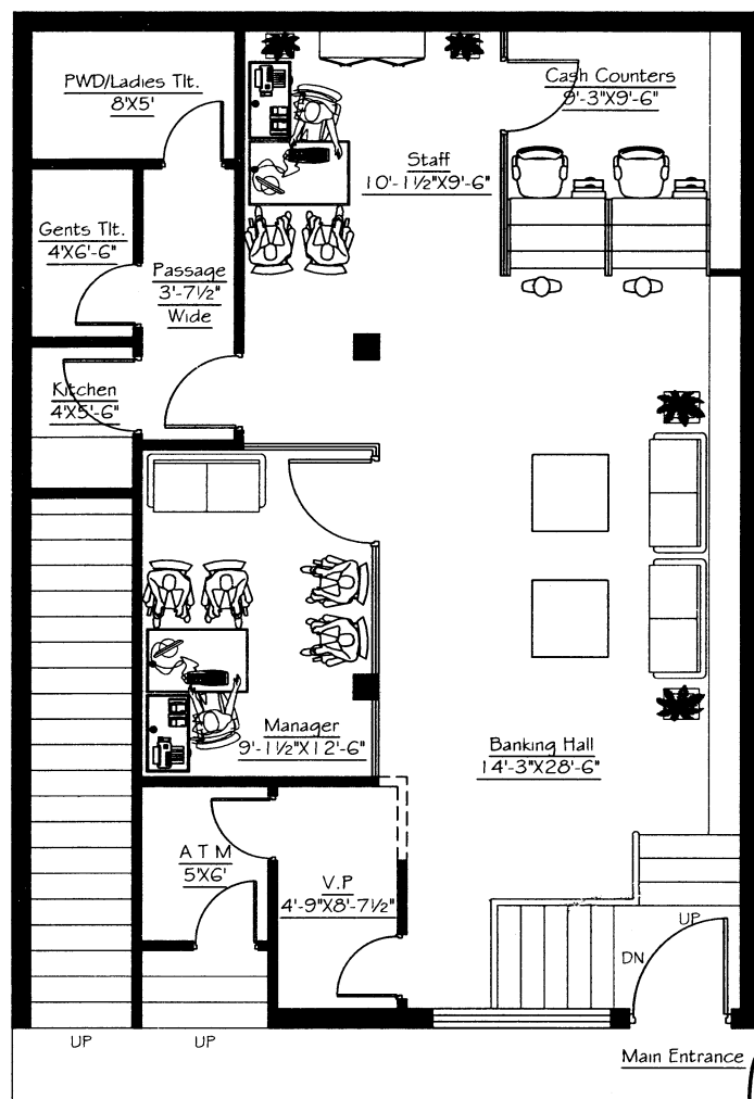
GROUND FLOOR PLAN 1,165 SQ.FT
