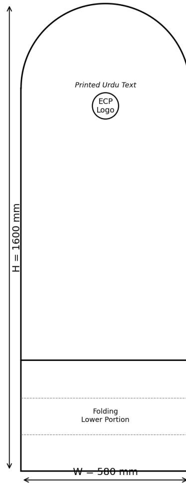
FRONT ELEVATION
