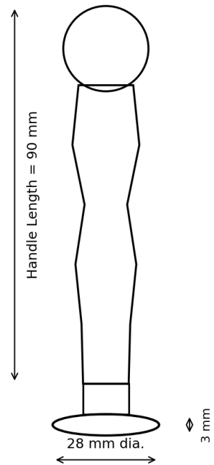
SIDE ELEVATION
