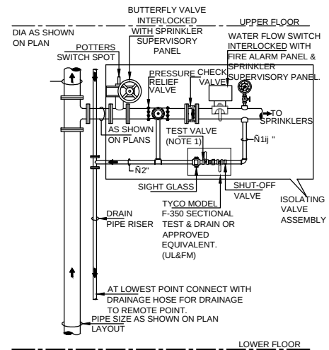
ZONE CONTROL VALVE WITH PRV ASSEMBLY DETAIL
