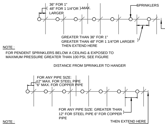
DISTANCE FROM SPRINKLER TO HANGER
