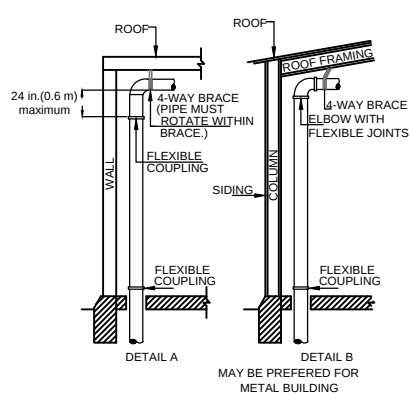
RISER DETAIL
