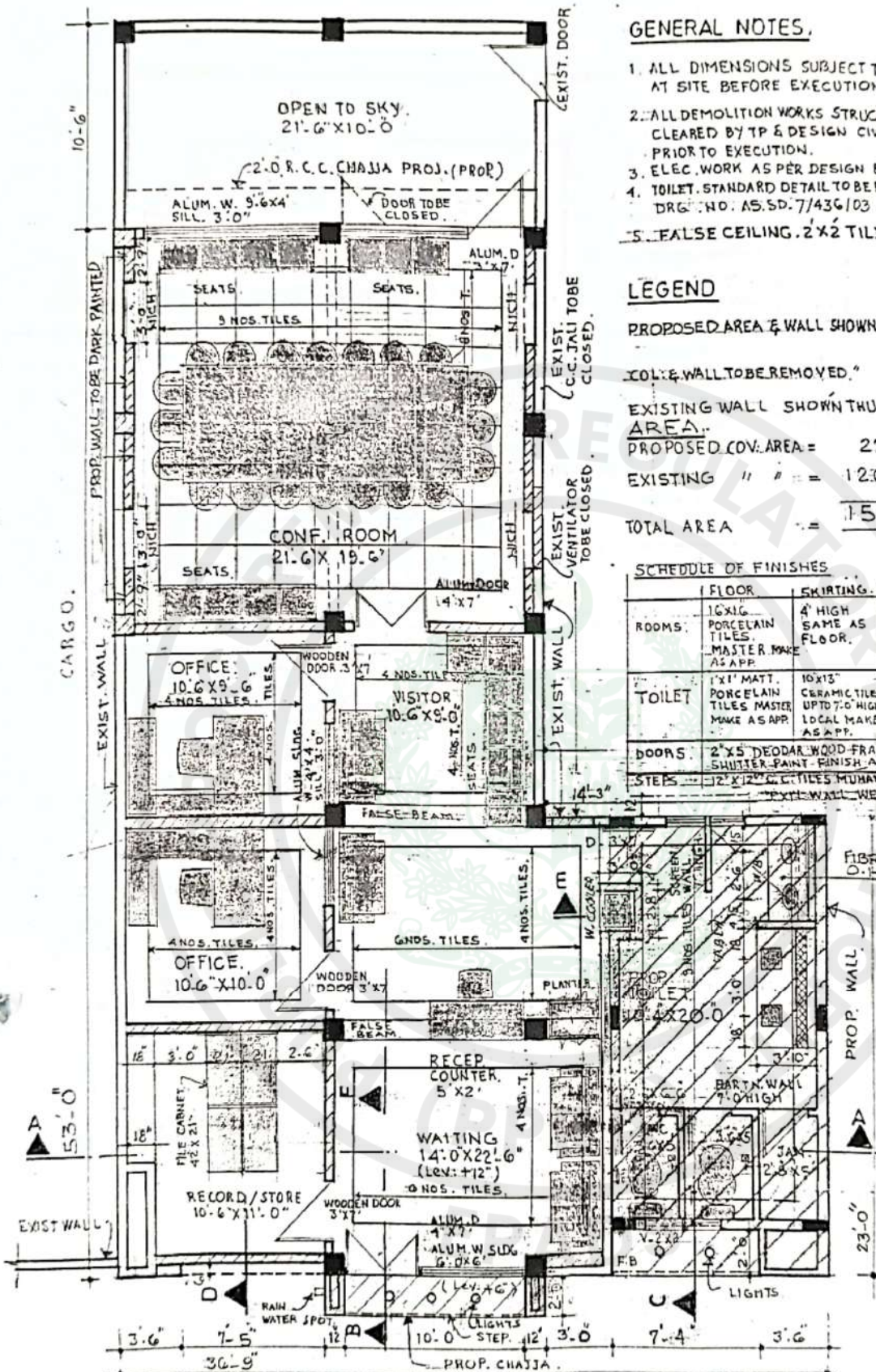
PLAN SCALE: 3/16" = 1'-0"
