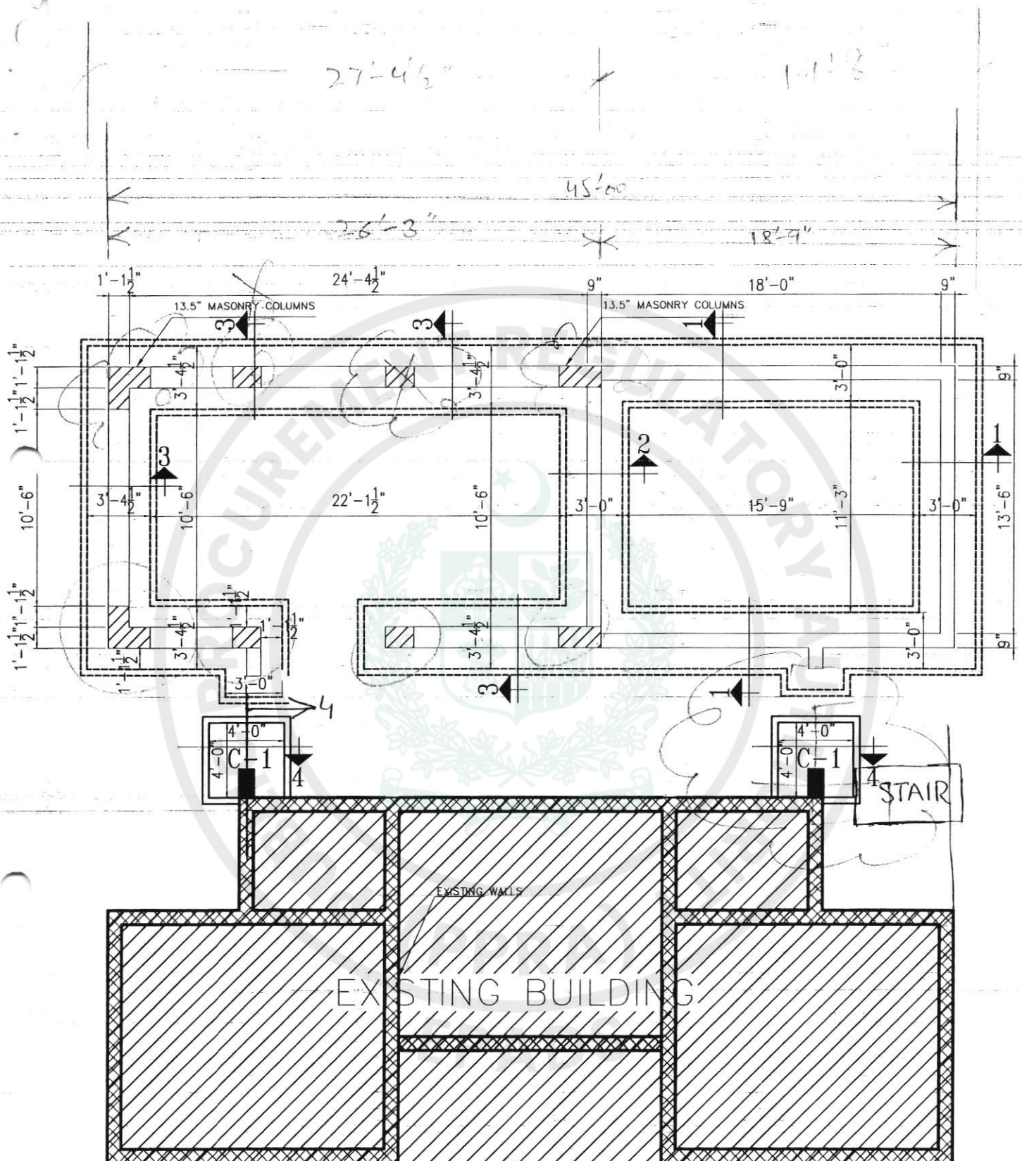
FOUNDATION LAYOUT PLAN
