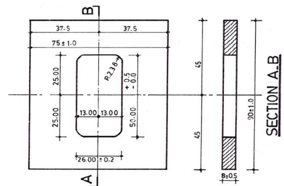
PLAN SCALE FULL SIZE
