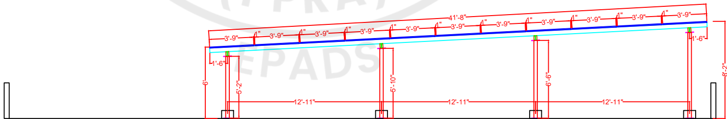
RIGHT VIEW
