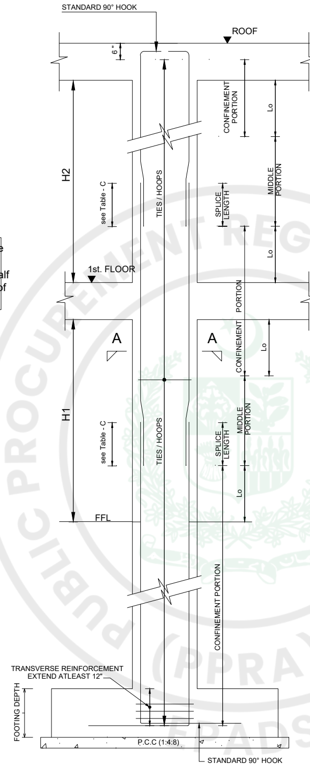
TYPICAL MULTI STORY COLUMN DETAILS
