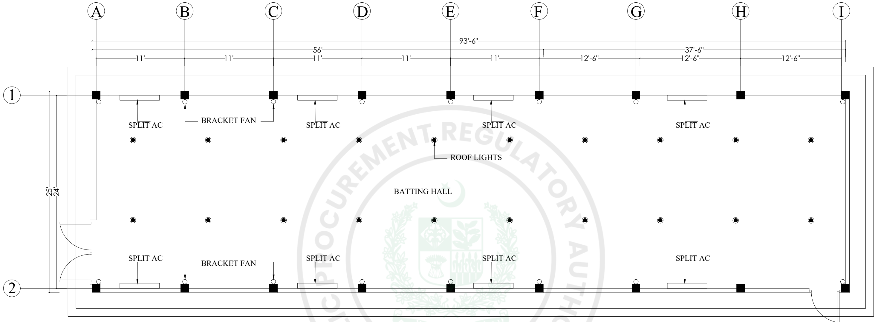
GROUND FLOOR LIGHTING PLAN
