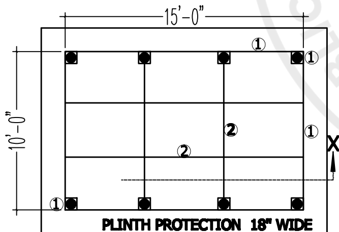
PLAN ( SHED)
