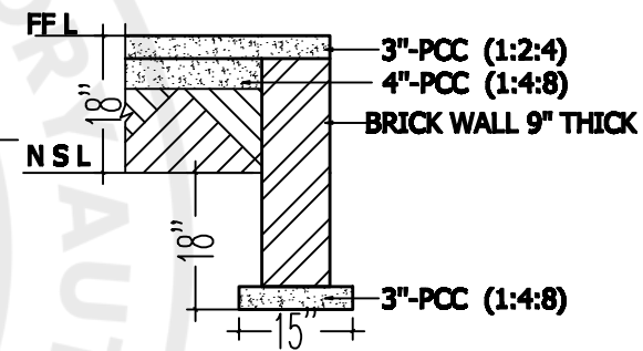
TOE WALL SECTION
