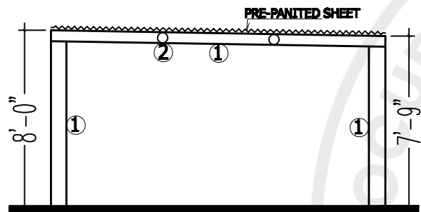
SECTION -X
