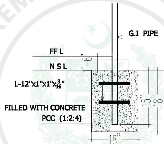
TYPICAL SECTION
