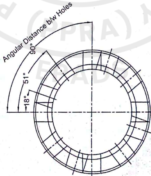
BUSH FOR CNR # 05
