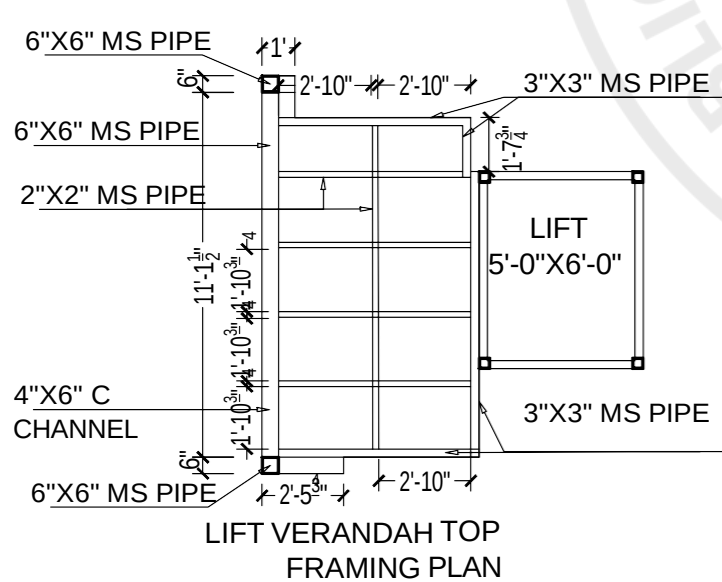
LIFT AND VERANDAH PLAN
