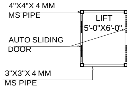
LIFT FRAMING PLAN
