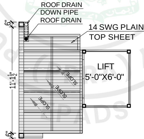
LIFT AND VERANDAH PLAN
