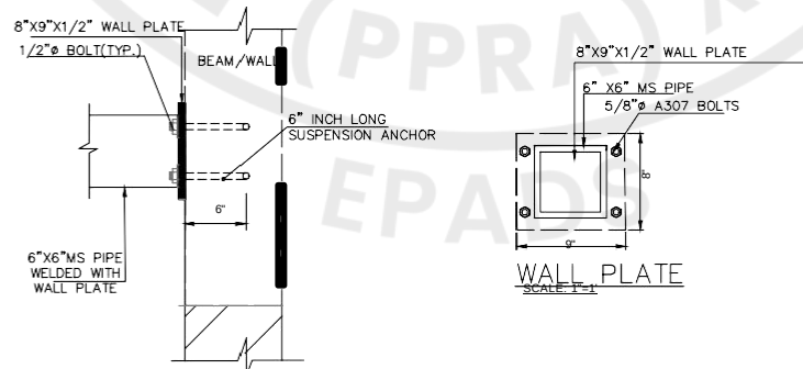
SECTIONAL ELEVATION OF WALL PLATE CONNECTION
