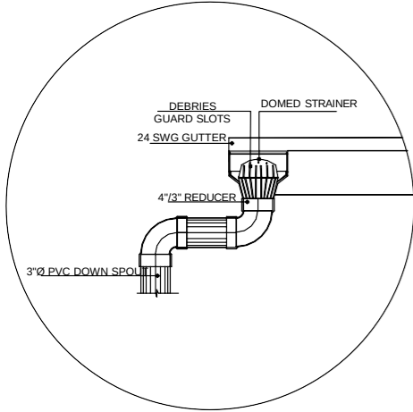
SECTION: 1-1 SCALE: 3/4"=1'
