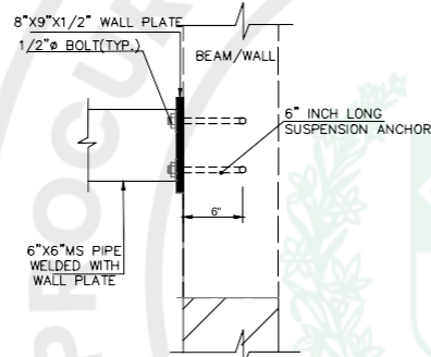
SECTIONAL ELEVATION OF WALL PLATE CONNECTION
