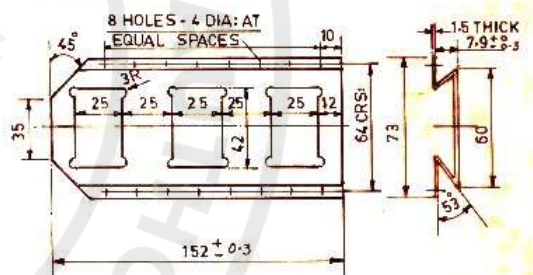
DETAIL OF SUPPORT PLATE
