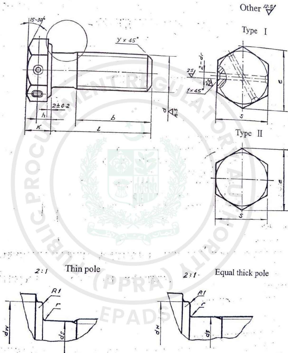
Fig. 1 the axle end bolt of the locomotives and cars
