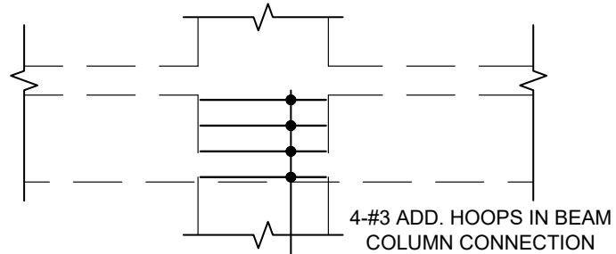
DETAIL 'X'
