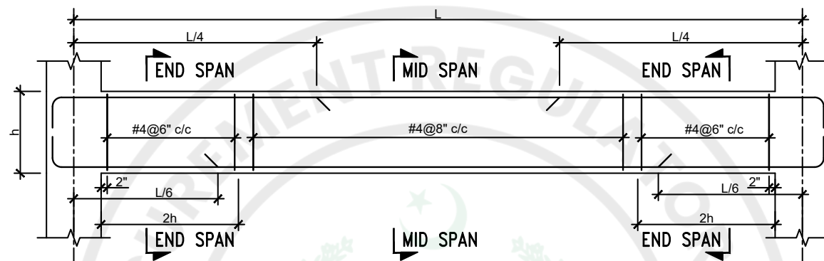
Typ. BEAM ELEVATION
