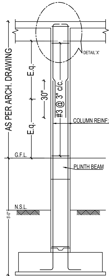
Typ. COLUMN ELEVATION
