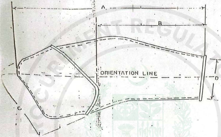
FIG. 1 STYLE B CURVED ELBOW SLEEVE
