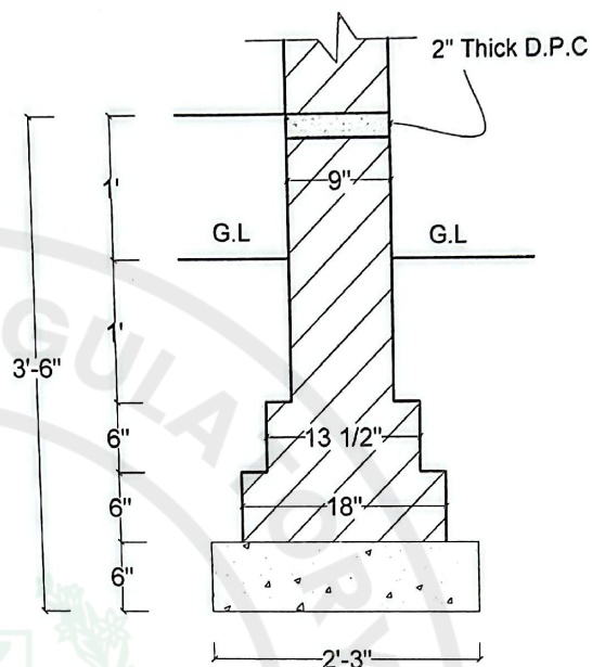
FOUNDATION DETAIL
