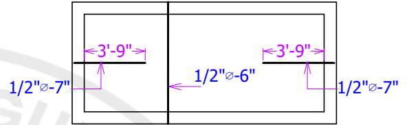
SLAB ROOM (TOP BARS)
