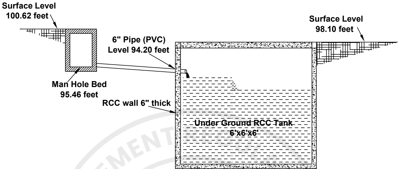
EXISTING STRUCTURE WETLAND TANK (HYBRID) UNDER GROUND
