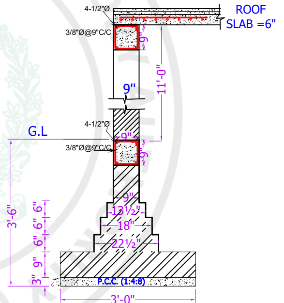
SECTION AT 3-3
