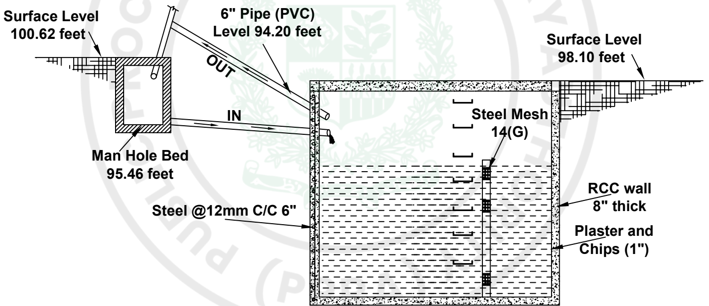
SECTION (A-A) WETLAND TANK (HYBRID) UNDER GROUND
