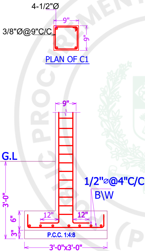
X SECTION AT A-A
