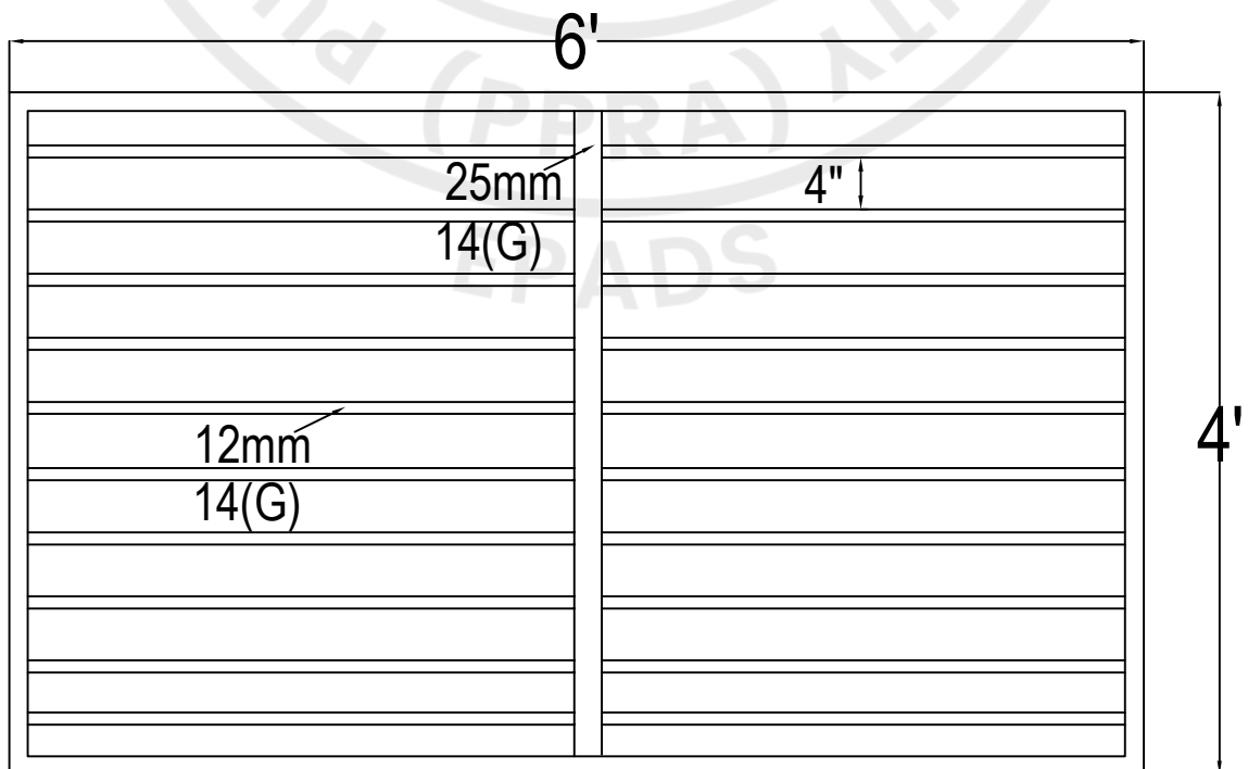
WINDOW IRON GRILL
