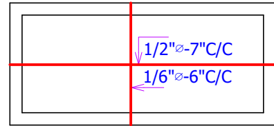
SLAB REINFORCEMENT PLAN OF ROOM (BOTTOM BARS)
