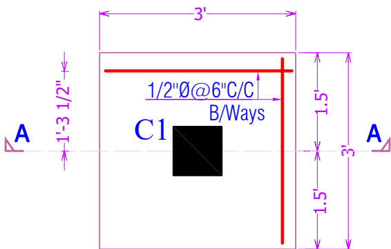
PLAN OF F-1
