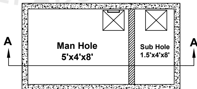
PROPOSED WETLAND TANK (HYBRID) UNDER GROUND
