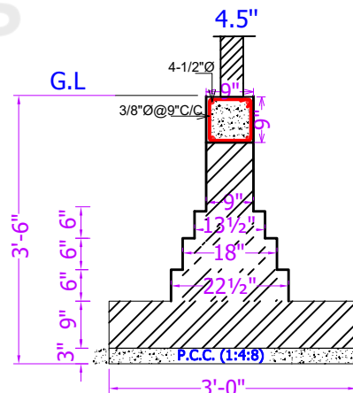
SECTION AT 2-2
