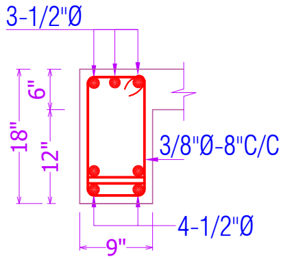
X. SECTION OF C-2
