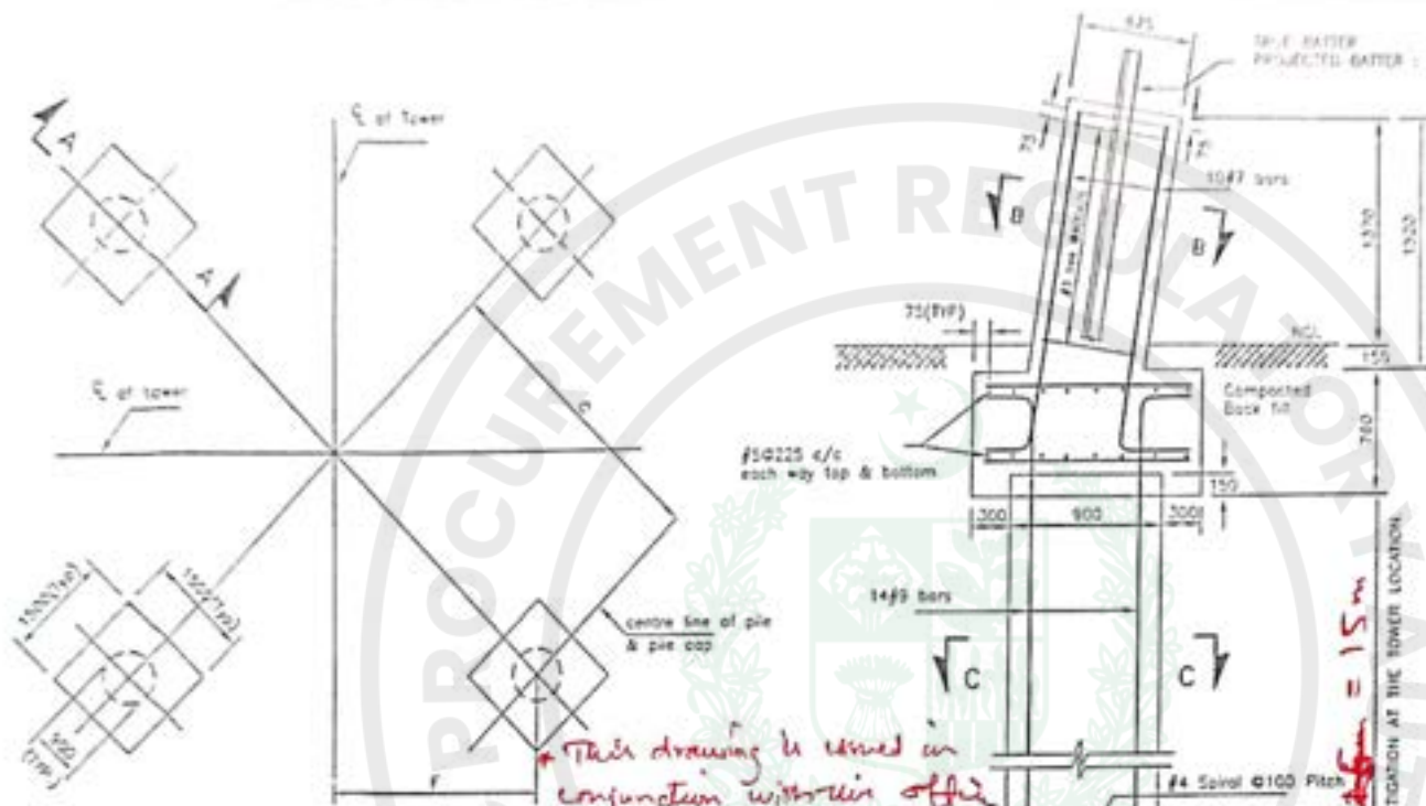
PLAN AT TOP OF PILE CAP PAD
