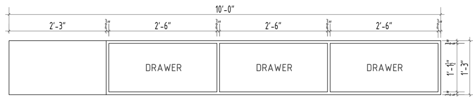
CONSOLE PLAN (DETAIL-01)
