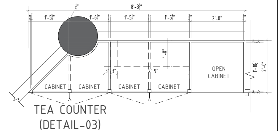
ELEVATION (DETAIL-03)
