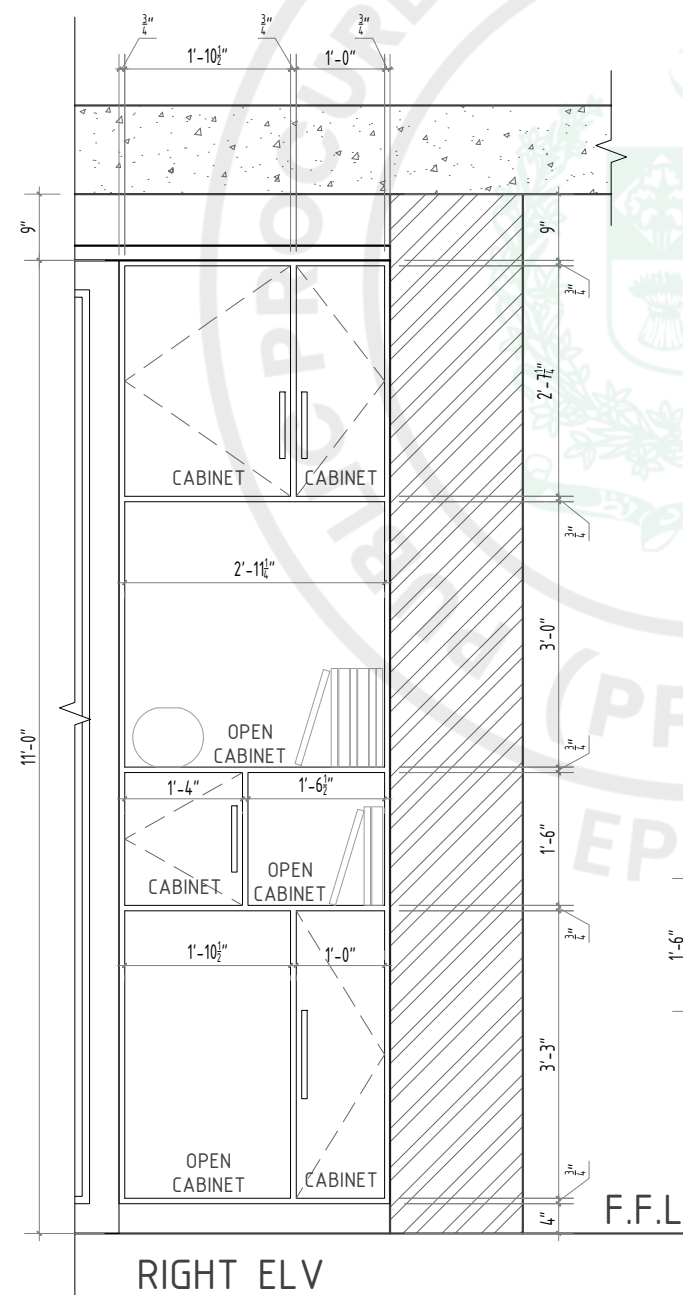
STORAGE & DISPLAY UNIT (DETAIL-02)
