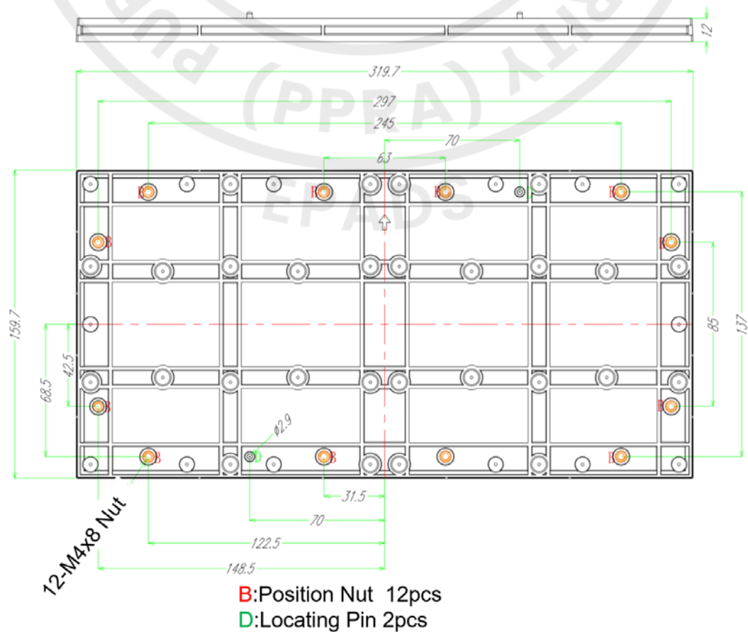
Picture 4-1 Hole Installation Diagram for Kit
