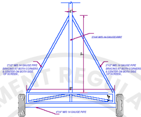
BASE STRUCTURE SIDE ELEVATION
