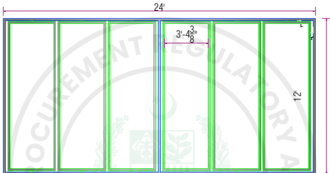
CRICKET SIGHT SCREEN ELEVATION
