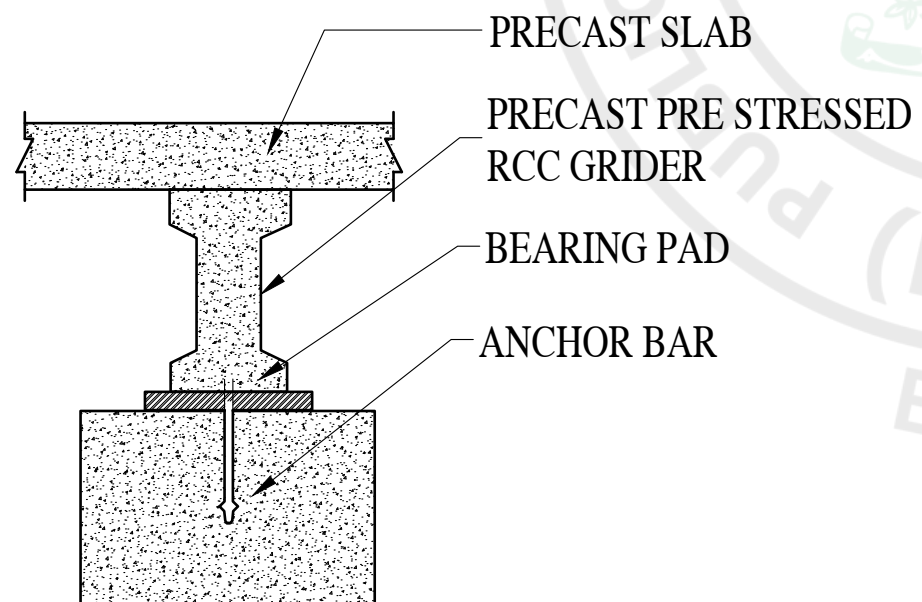
GRIDER BEARING ANCHORAGE DETAIL
