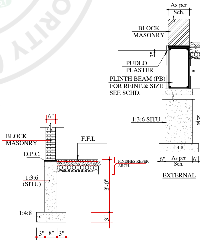
TYP. SEC. OF WALL FOOTING
