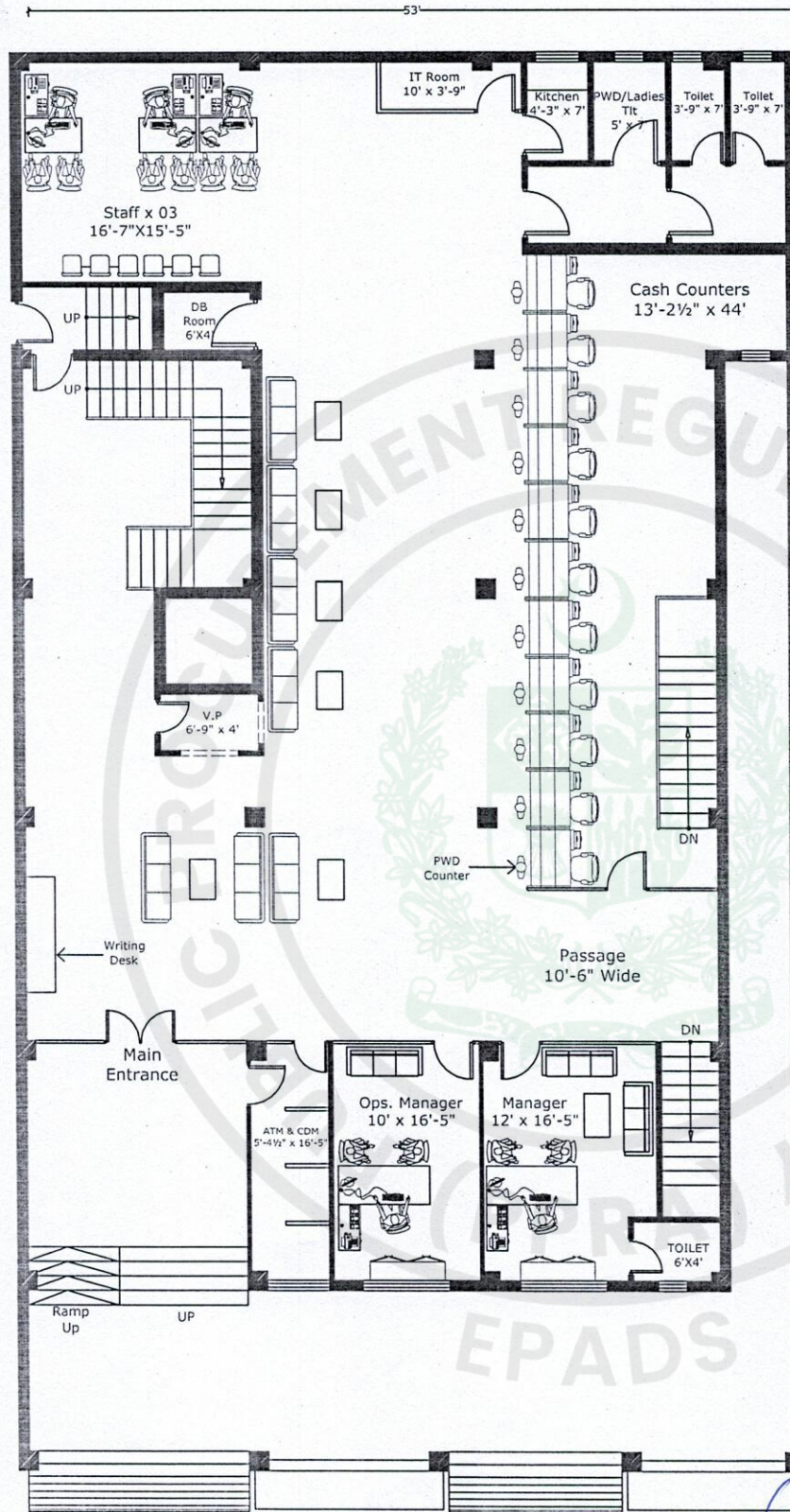
Ground Floor Layout Plan
