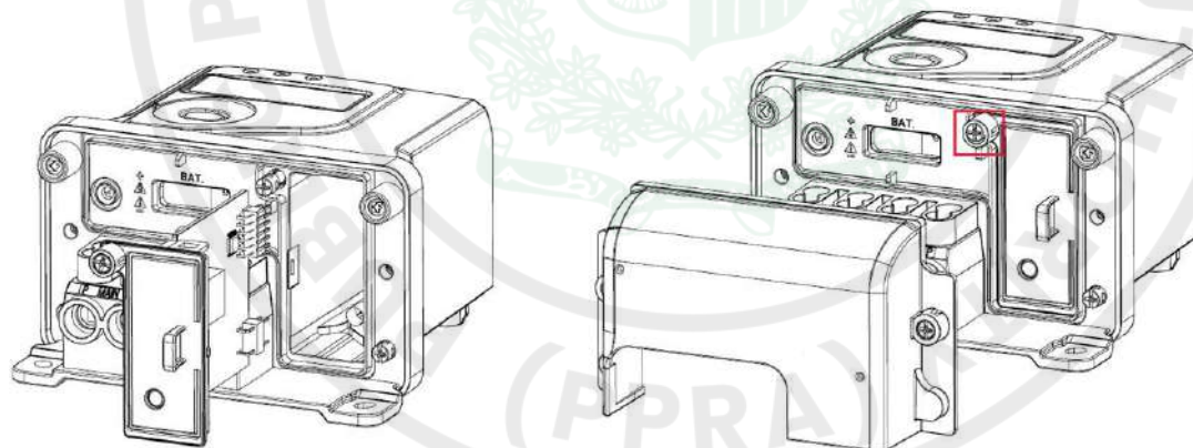
Figure - 2 Mounting for Single-phase meter
