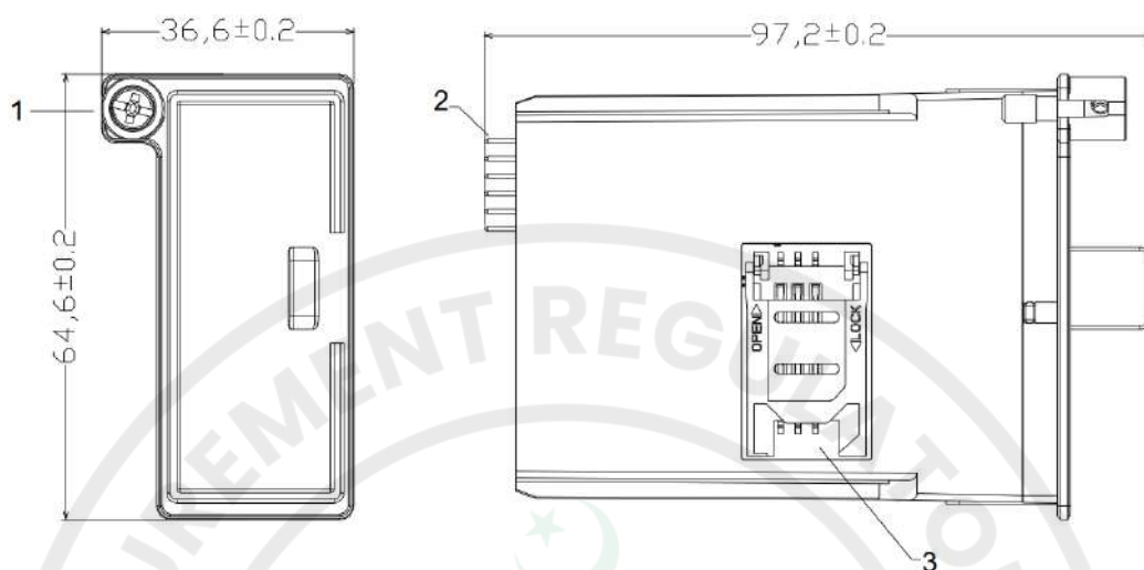
Figure - 1 General view of 4G/2G module
