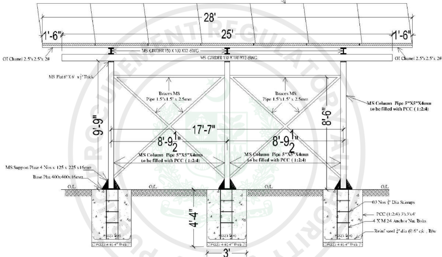
Front Elevation / Section
