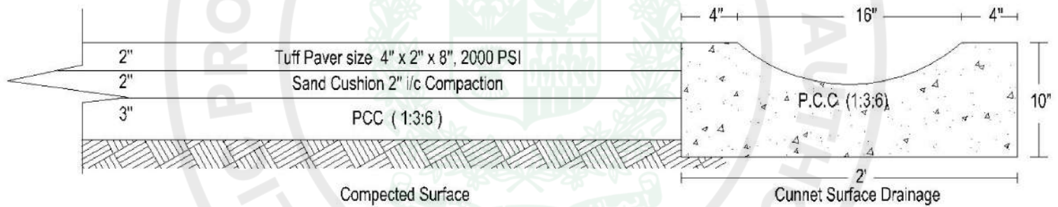
Drawing # 5 Section
